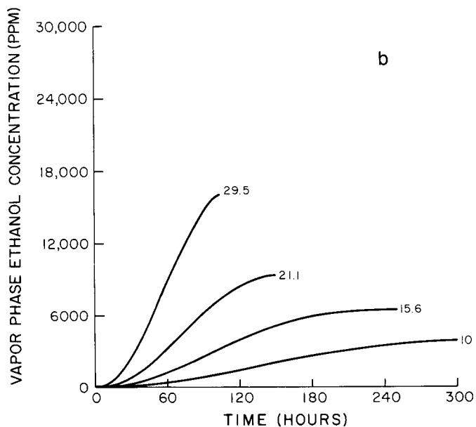
Fig. 7. The influence of fermentation temperature on a) the fermentation rate, b) the vapor phase ethanol concentration, and c) the rate of ethanol emission. (Initial sugar content of 22.5°Brix, isothermal fermentation at indicated temperature.)
